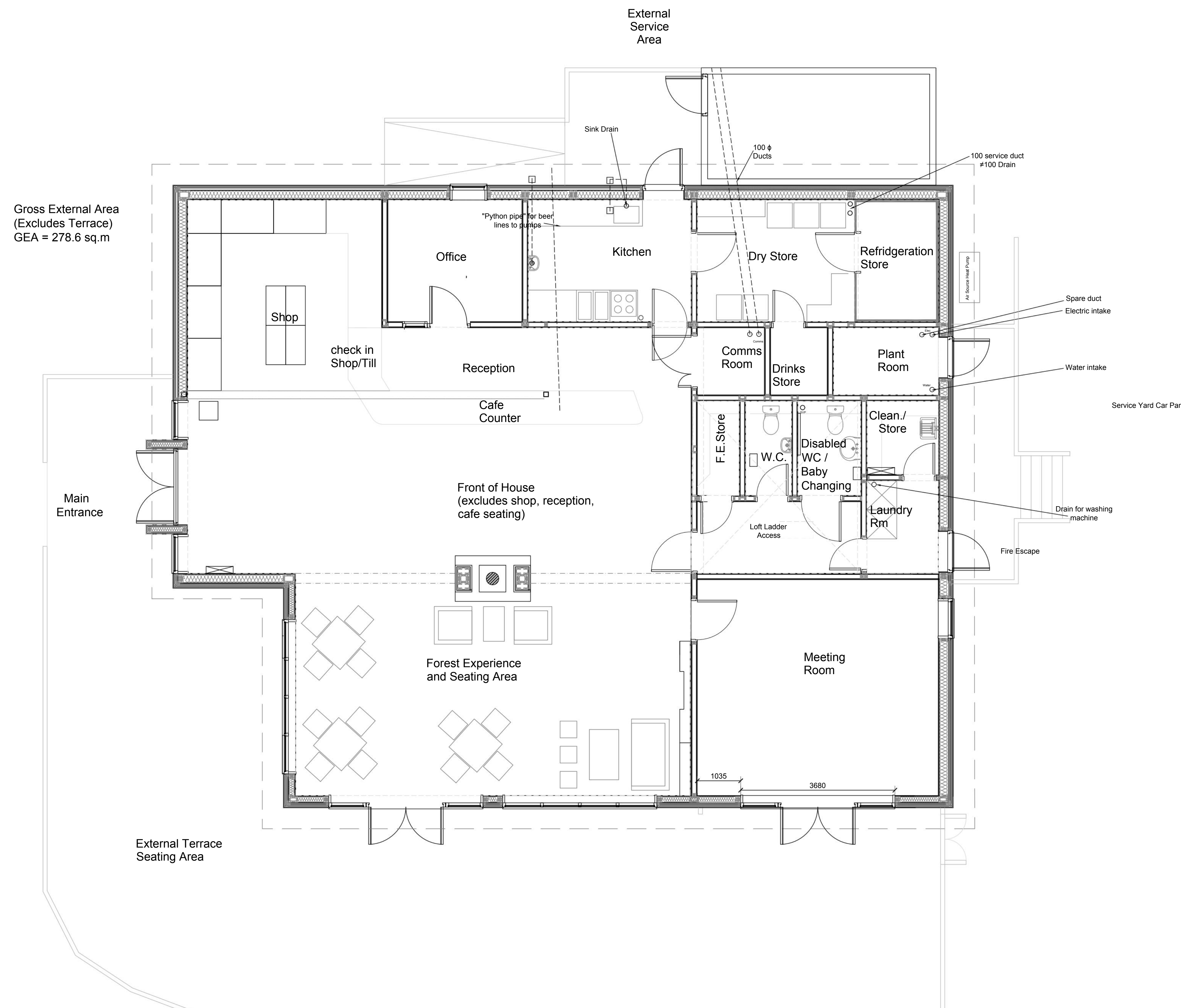
01 GROUND FLOOR PLAN Scale: 1:50 (A1)
