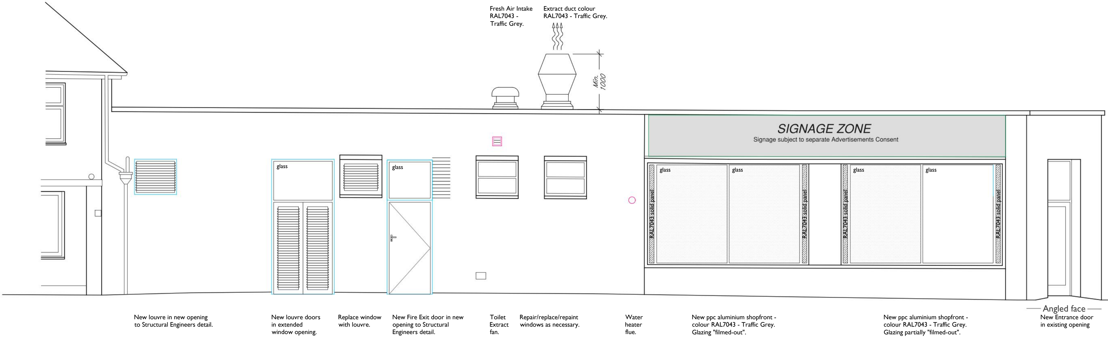
PENDLEFORD MILL LANE ELEVATION - South
