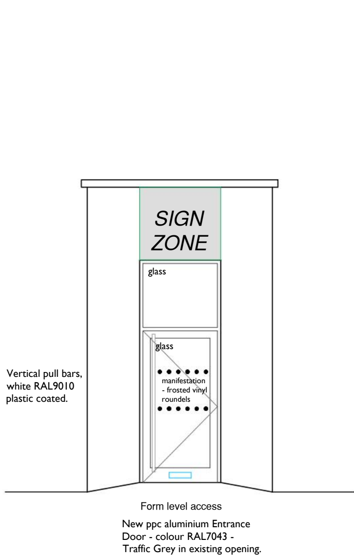
ENTRANCE ELEVATION - South East
