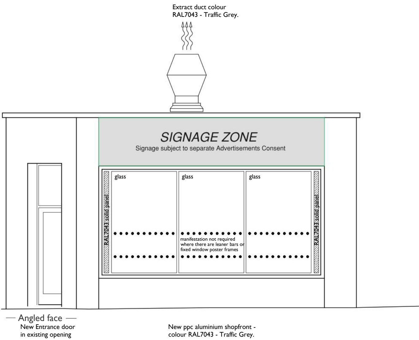
LANE GREEN ROAD ELEVATION - East
