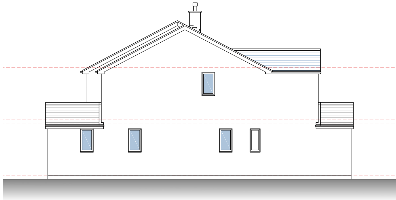
Right Side (South) Elevation
