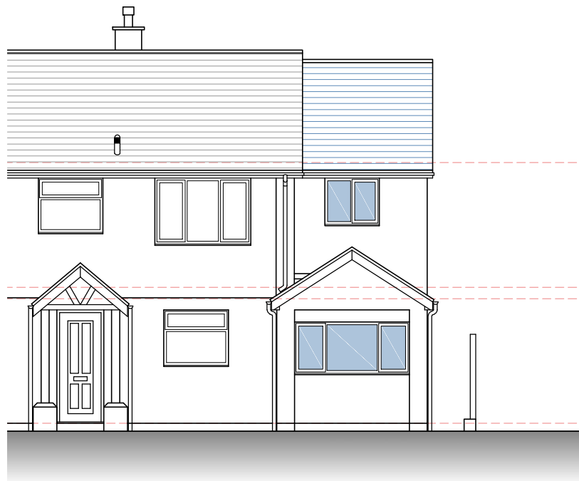
Front (West) Elevation
