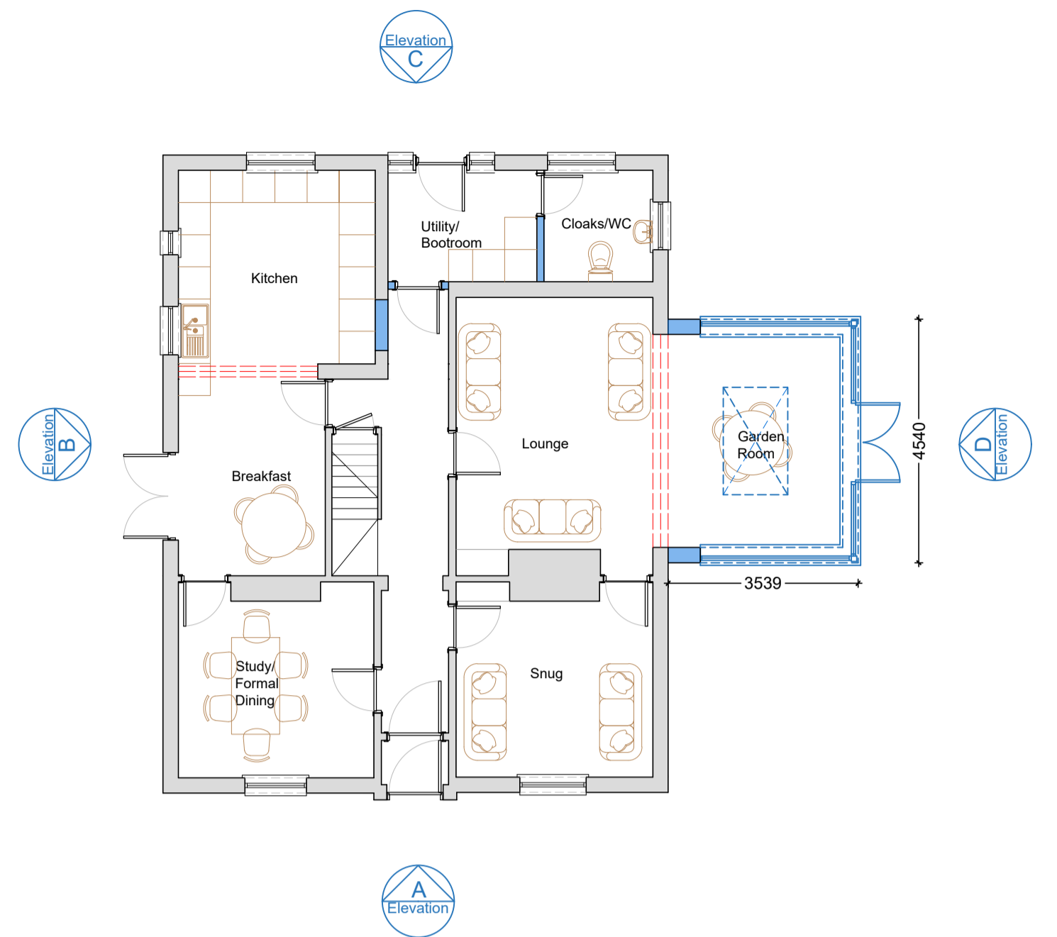
Proposed Ground Floor Plan 1:100 Scale
