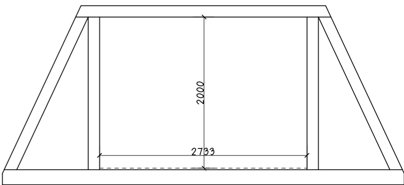
Proposed 'Gambrel' Attic Truss
